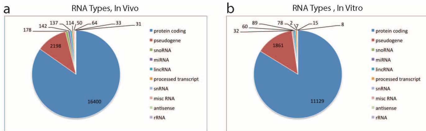
Extended Data Figure 6 | icSHAPE is capable of measuring the RNA structure profiles of thousands of RNAs simultaneously. a, The RNAs represented in polyA-selected RNA, in vivo . b, The RNAs represented in polyA-selected RNA, in vitro .
