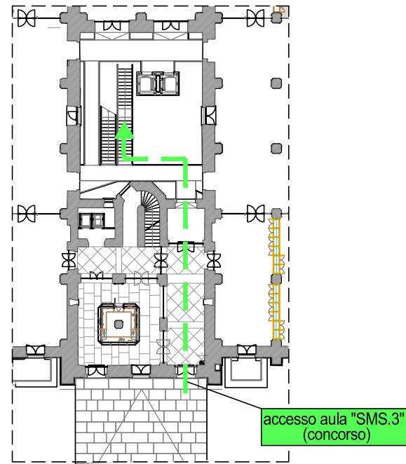
PIANO TERRA
